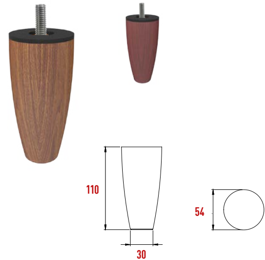
R223 Nevada Ayak 110 mm
