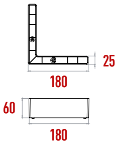
T212 Seat Köşe Ayak 180x180x60 mm
