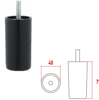
P988 Forte Gizli Ayak 77mm
