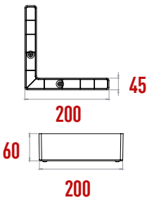
S151 Seat Köşe Ayak 200x200x60 mm
