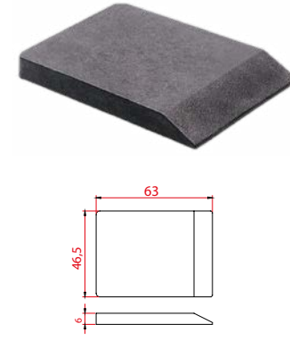
P1312 Döşeme Yan Pls.
