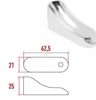
P3087 Opera Zigon Sehpa Ayağı
