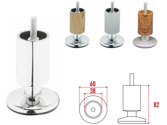
P905 Fullex Ayak 82 mm
