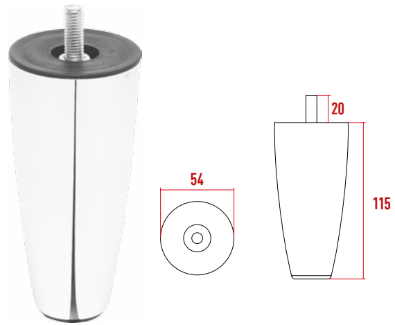
P856 Nevada Ayak 115 mm
