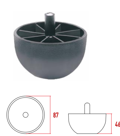
P1075 Hukla Ayak Pimli
