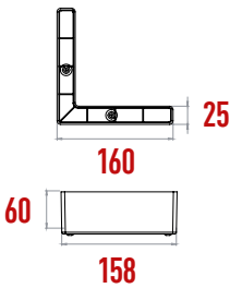
T172 Seat Köşe Ayak 160x160 mm
