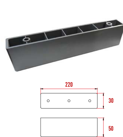
Y383 Kingstone Ayak 220x50 mm
