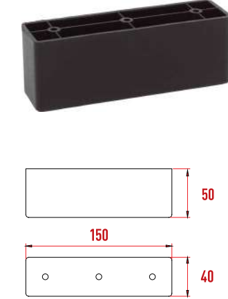
Y382 Kingstone Ayak 140x50 mm
