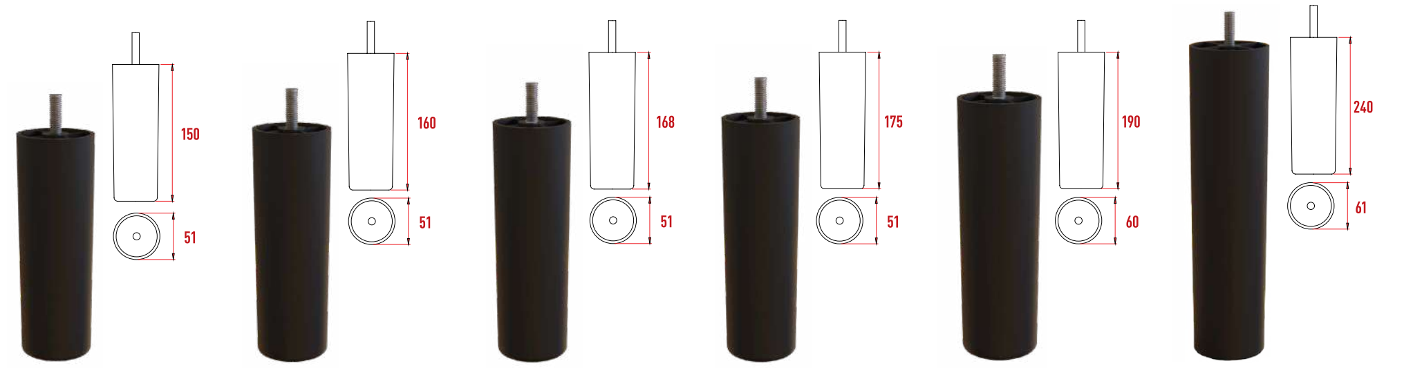
P855 Arizo Ayak 150 mm Y508 Gizli Ayak 160 mm Y793 Gizli Ayak 168 mm Y506 Gizli Ayak 175 mm R257 Arizo Ayak 190 mm Y880 Arizo Ayak 240 mm
