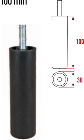
S115 Berlino Silindir Ayak 100 mm
