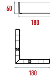
T212 Seat Köşe Ayak 180x180x60 mm
